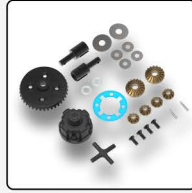
SAK-D501 39T METAL GEAR DIFFERENTIAL FOR D5S Sakura D5SHIギアアプテア39T
